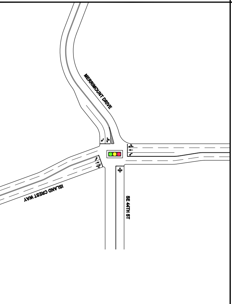
SIGNAL WITH TURN LANE: INSTALLATION OF TRAFFIC SIGNAL AND WIDENING NB AND SB APPROACHES
