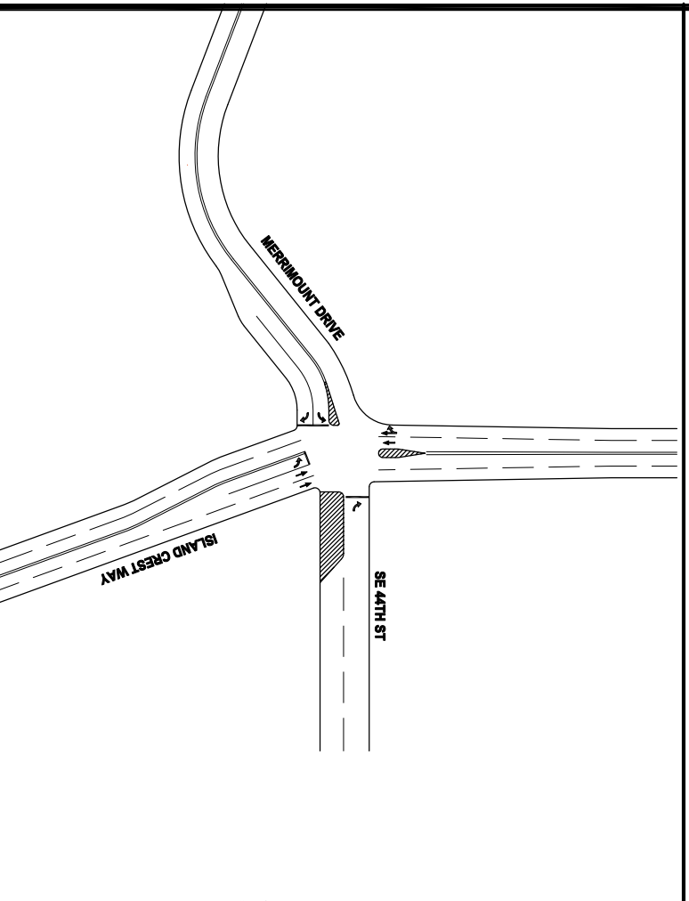
OPTION #5: WIDENING NB APPROACH AND RESTRICTION OF THROUGH MOVEMENTS AT ISLAND CREST WAY
