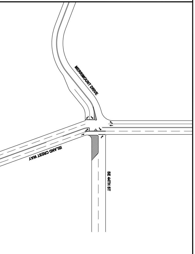
OPTION #4A - MODIFIED: RESTRICTION OF THROUGH MOVEMENTS AT ISLAND CREST WAY
