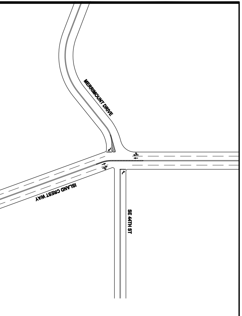
OPTION #1: RESTRICTION OF LEFT TURNS & THROUGH MOVEMENTS AT ISLAND CREST WAY
